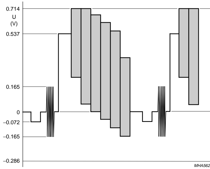
Fig.5 FCC/EIA colour bar 100% saturation, 75% amplitude with 12 dB sync attenuation.
